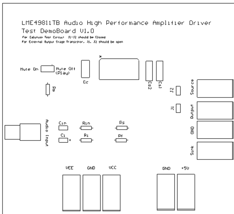
Figure 28. Silkscreen Layer
